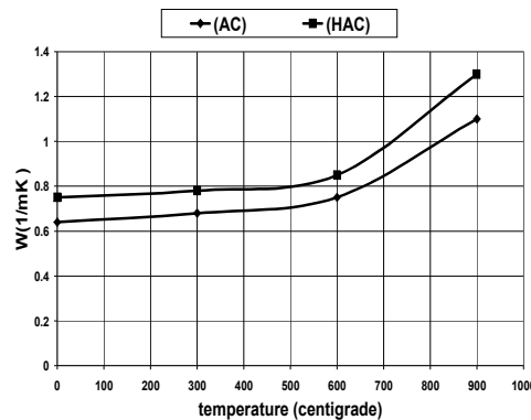
Figure 6. Coefficient of heat conductivity of alumina binder concrete in different temperatures
