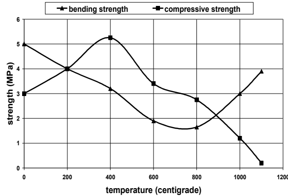
Figure 2. Variation of strength of silicate binder concrete with increase of the temperature
