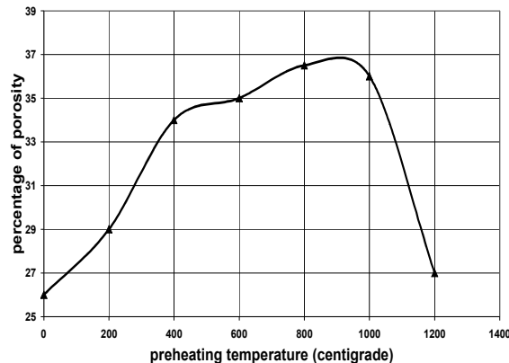
Figure 1. Effect of preheating temperature on percentage of porosity.
