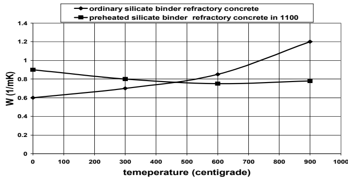
Figure 4. Coefficient of heat conductivity of silicate binder concrete in different temperatures
